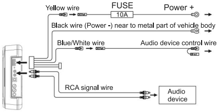
Wiring diagram 2 (Low level RCA input)
